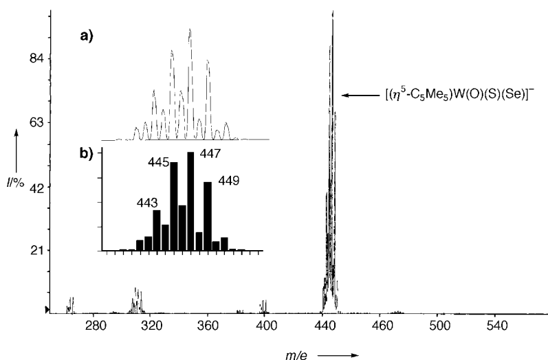
Figure 1. Negative ES mass spectrum of 3 in CH 3 CN; a) observed spectrum of the mass ion, b) theoretical isotope pattern.
